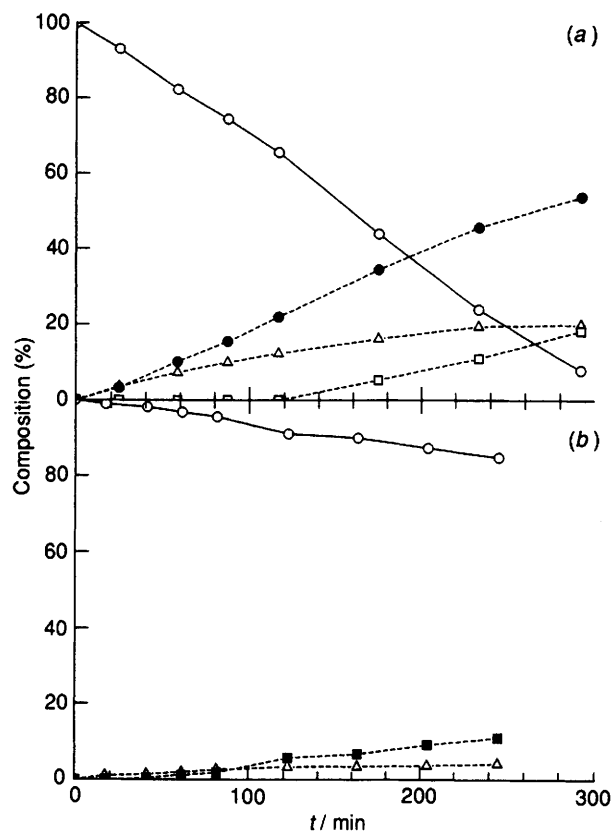
Fig. 1 Liquid-phase hydrogenation of cinnamaldehyde over alumina-supported platinum catalysts prepared by LLR for 30 min (a) and by HHR at 573 K (b). (O) cinnamaldehyde; (●) cinnamyl alcohol; ( \Delta ) hydrocinnamaldehyde; ( \square ) phenylpropanol; ( \blacksquare ) hydrocinnamaldehyde diethylacetal.
